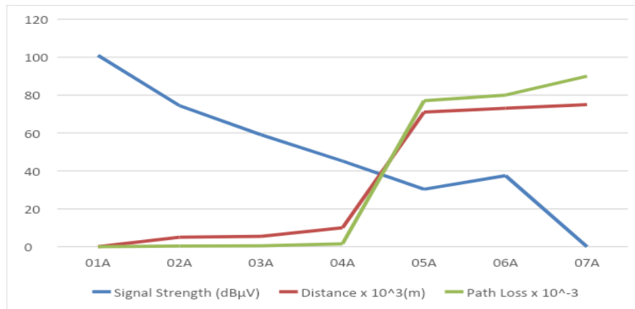
Fig. 3: Relationship between signal strength, distance and path loss for radio Kogi
