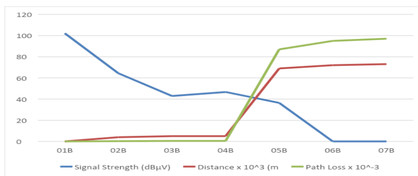
Fig. 4: Relationship between signal strength, distance and path loss for TAO FM
