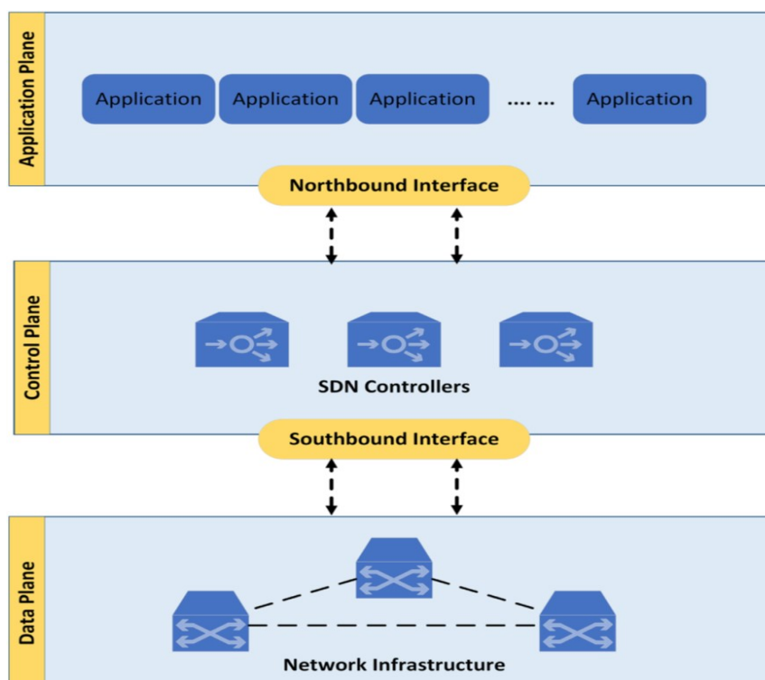
Fig. 1: SDN Architecture
