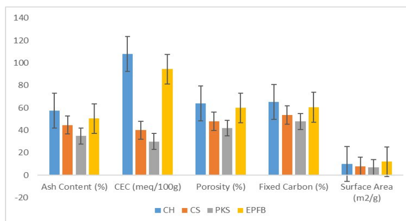
Figure 2: Surface Physicochemistry of Four Different Biochars Used for Heavy Metals Adsorption
