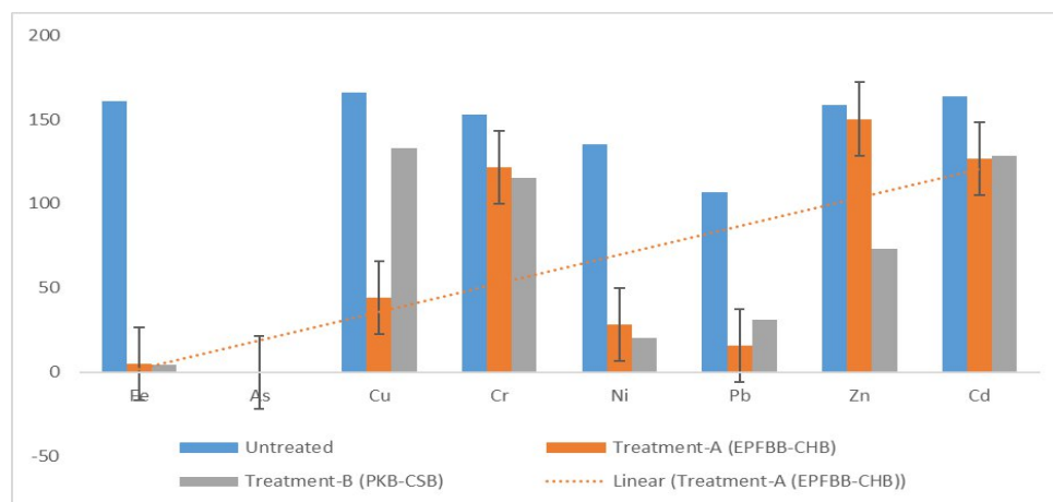
Figure 1: Treatment Performance of Two Biochar Composites for Heavy Metal Reduction in Soil
