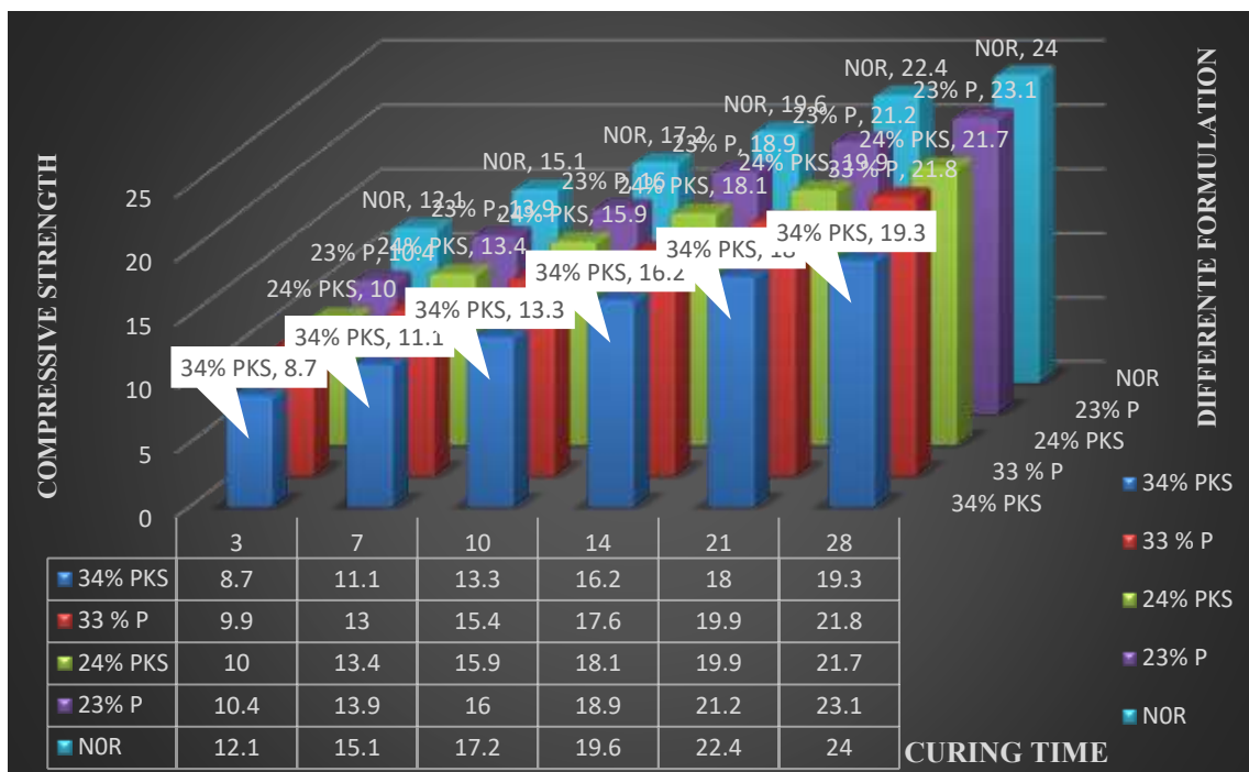
Figure 8: Comparative compressive strength of the formulations at 3, 7, 21 and 28 days
