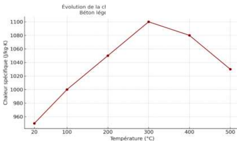
Figure 5: Evolution of the specific heat capacity of lightweight concrete based on the palm kernel shell as a function of temperature (Source: Anowai, 2023).
