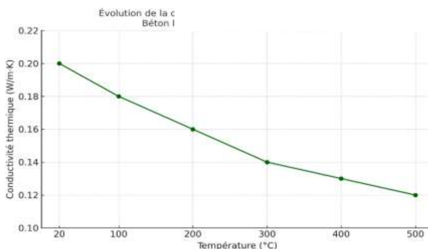
Figure 4: Evolution of the thermal conductivity of lightweight concrete based on palm kernel shell versus temperature (Source: Anowai, 2023).
