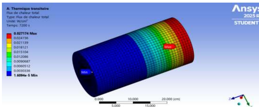
Figure 17: Heat flux distribution in the 34% PKS concrete formulation after 7200 seconds
