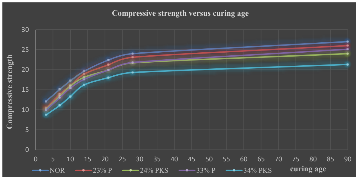
Figure 7: Variation of compressive strength with curing age for all formulations
