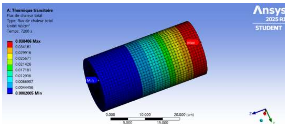
Figure 17: Heat flux distribution in the 34% PKS concrete formulation after 7200 seconds
