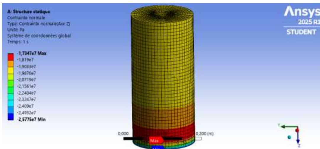
Figure 10: Normal stress distribution in concrete with 34% palm kernel shell under axial load ANSYS static structural simulation
