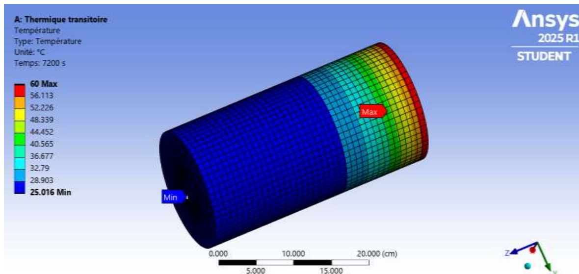
Figure 13: Transient thermal simulation in ANSYS showing heat propagation in 34% PKS concrete after 7200 seconds
