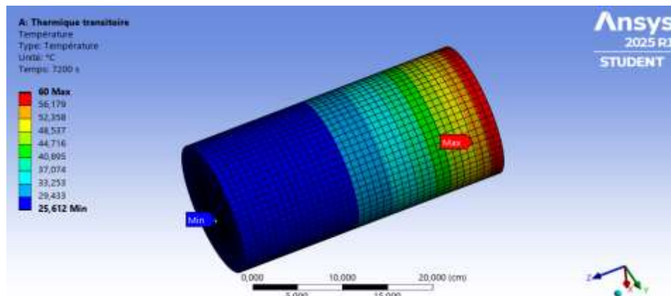
Figure 12: Transient thermal simulation in ANSYS showing heat propagation in 33% pozzolan concrete after 7200 seconds
