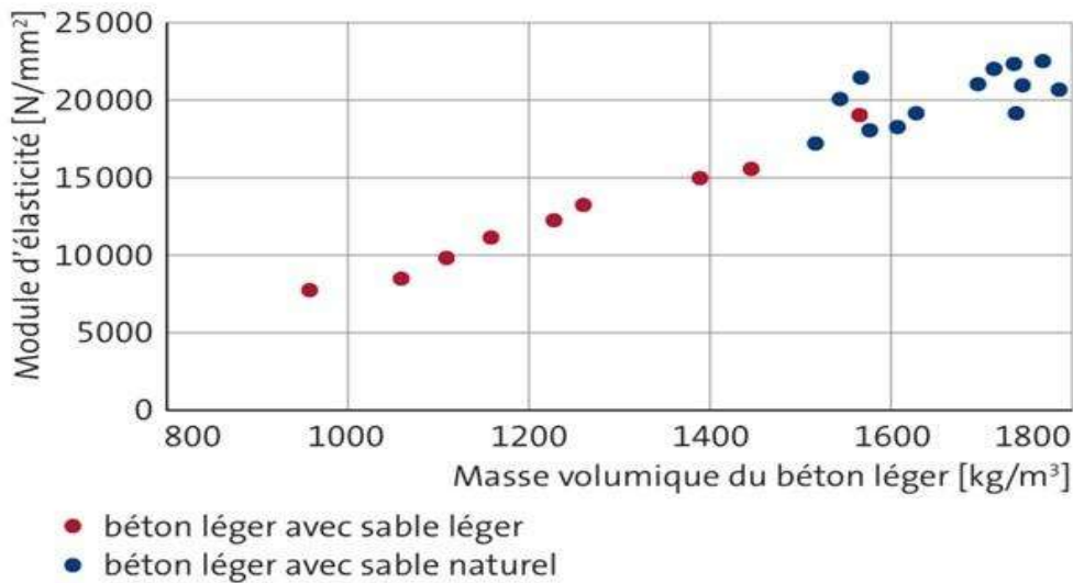
Figure 3: Relationship between the dry density and the modulus of elasticity for various types of lightweight concretes (Source: Dr. Peter Lunk, 2015)
