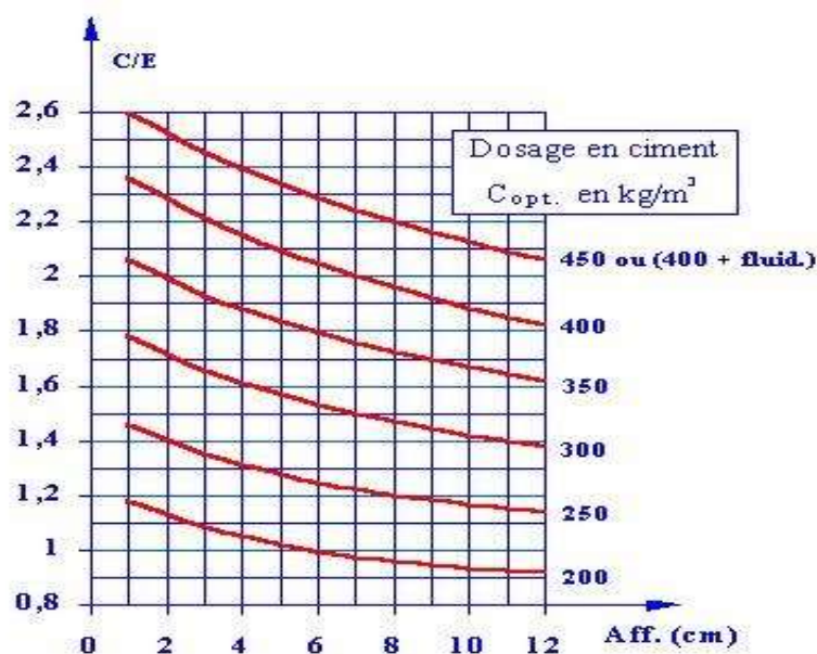
Figure 6: Chart for determining C_{\text{opt}} (Source: Yousfi, 2016)
