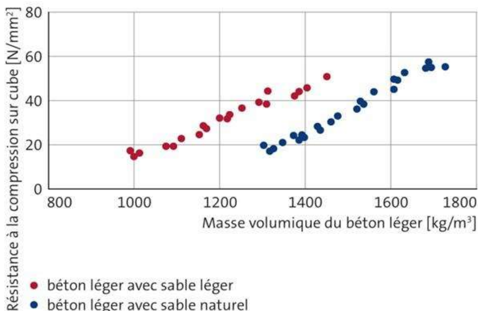
Figure 2: Variation of compressive strength with bulk density (Source: Dr. Peter Lunk, 2015)
