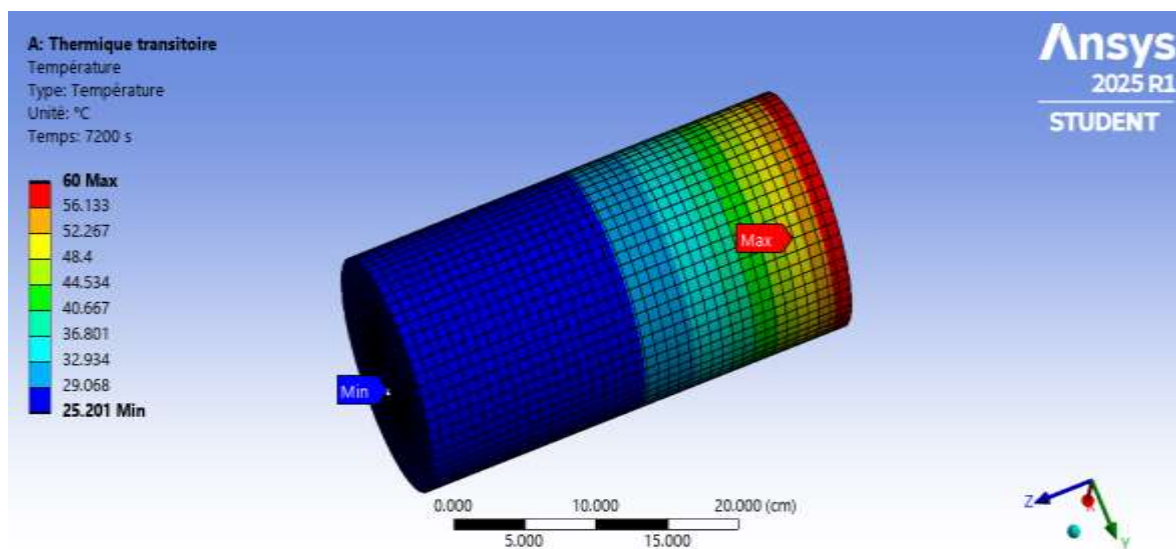
Figure 12: Transient thermal simulation in ANSYS showing heat propagation in 33% pozzolan concrete after 7200 seconds
